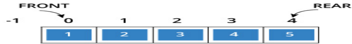
EnQueue
